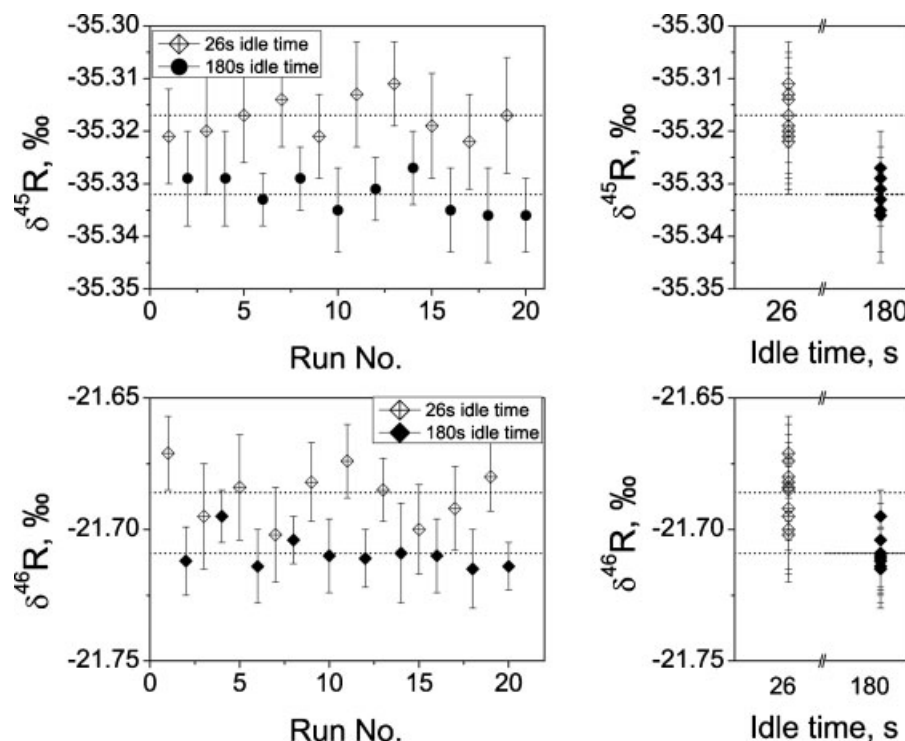
Figure 1. \delta^{45}\text{R} and \delta^{46}\text{R} values obtained with idle times of 26 s (○) and 180 s (●) in fully symmetrical DI mode (shown are 2- \sigma values, internal precision). The discrepancy of 0.015‰ and 0.020‰, respectively, is observed for the large isotope difference between two gases ( -35.33 and -21.71\text{‰} in \delta^{45}\text{R} and \delta^{46}\text{R} , respectively). The corrections for air samples analysed vs. WR-CO 2 are \sim 0.001\text{‰} and 0.007\text{‰} , respectively.
