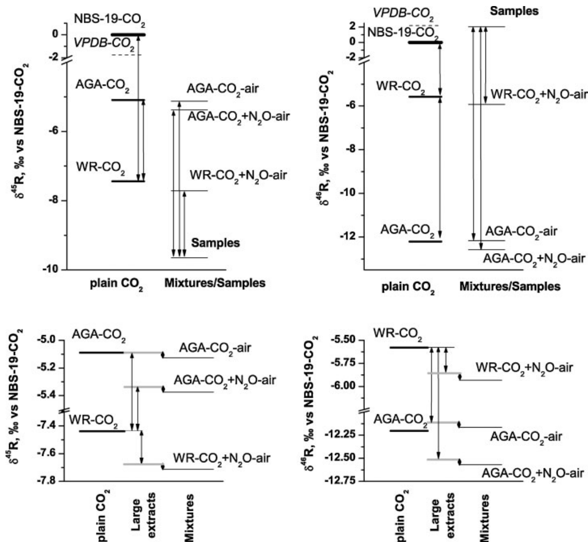
Figure 8. The approach of using mixtures based on 'known' CO 2 with and without N 2 O doping. The upper panel shows the calibration on plain CO 2 gases and air samples vs. CO 2 -air mixtures. Here the calibration link between plain CO 2 and CO 2 -air mixtures is missing. The lower panel shows practical realisation of this link by using large extracts from the mixtures analysed in DI mode; the distance between each mixture and large extracts (small arrows) gives a correction magnitude. Other distances have also been measured, proving our calibration approach.
