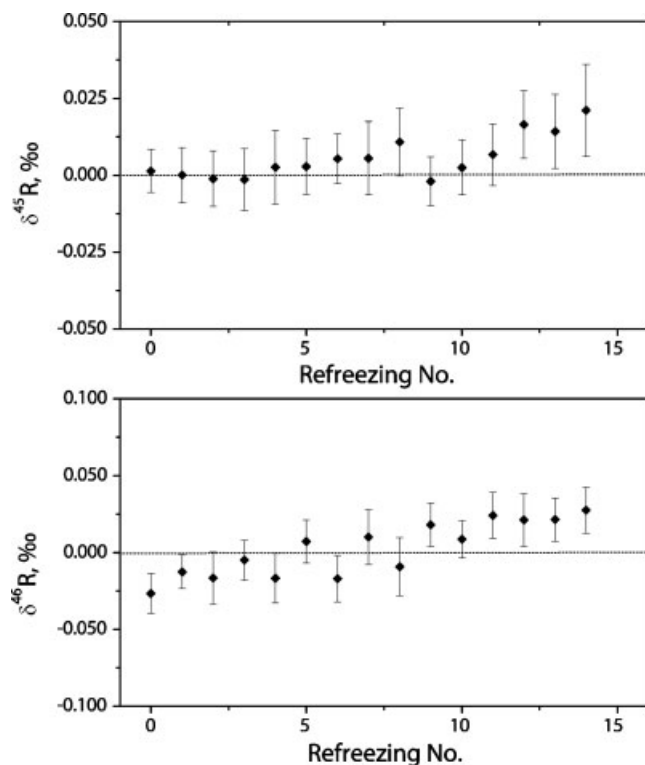
Figure 3. The effects of several freeze/thaw cycles of WR-CO 2 admitted to the cold trap on δ 45 R. Shown are 1-σ values. 0 and 7 correspond to runs without refreezing. The horizontal line shows the expected values for this (original) CO 2 . Given are 2-σ values based on 20 changeovers (internal precision).
