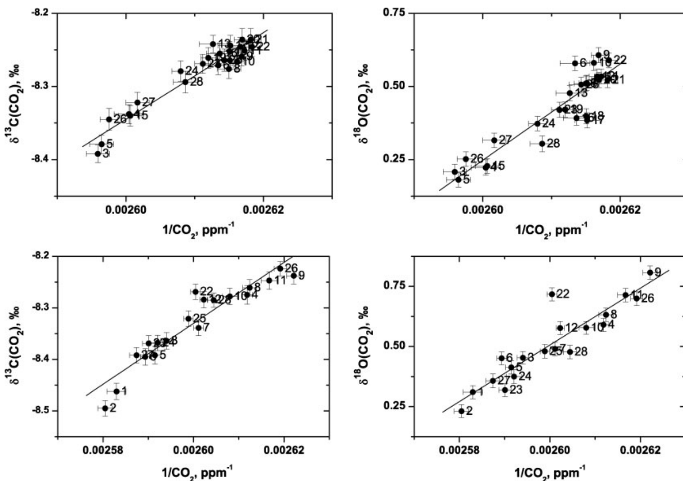
Figure 9. Some CARIBIC flights demonstrate a tight correlation between \delta^{13}\text{C}(\text{CO}_2) , \delta^{18}\text{O}(\text{CO}_2) and the CO 2 concentration (labels correspond to sample numbering in a flight, from 1 to 28). This implies a two end-member mixing, despite the long distances covered by the flights and the different air masses sampled over a route. Variabilities relative to the trend lines are used to give (over)estimations of total errors (analytical errors in CO 2 concentrations, isotope analyses, sampling quality and storage, etc.).
