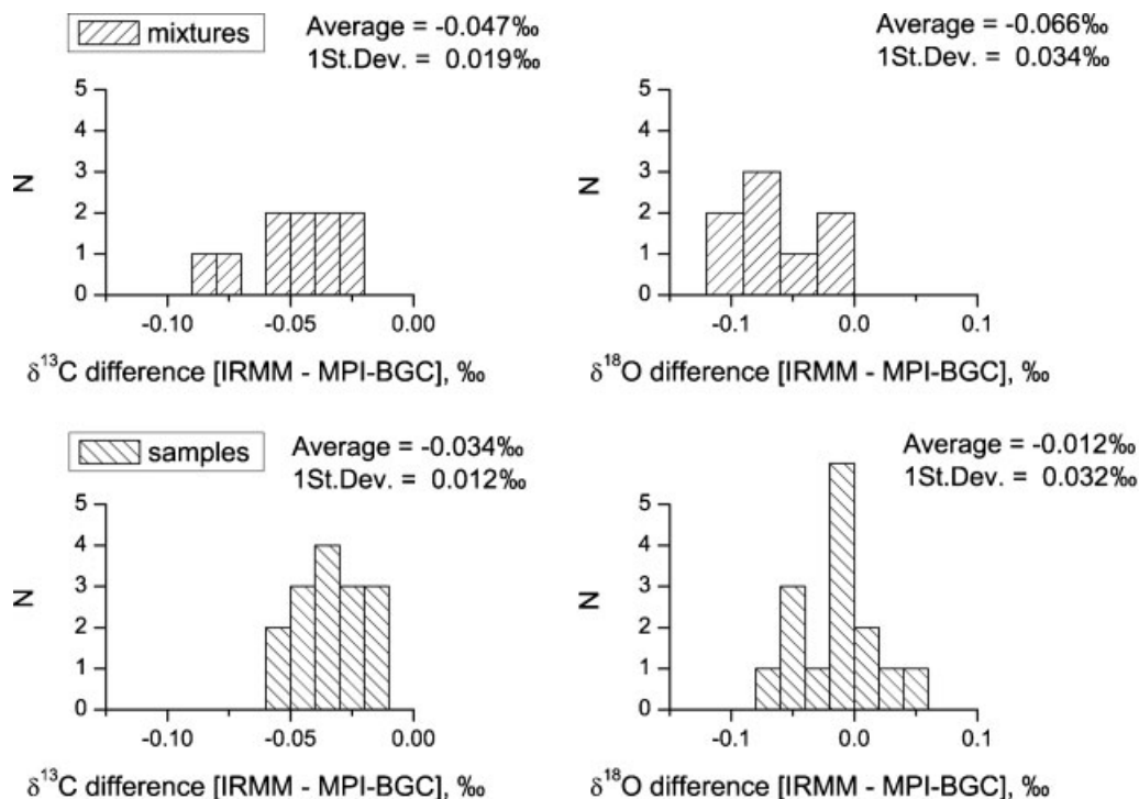
Figure 7. A difference in \delta^{13}\text{C}(\text{CO}_2) and \delta^{18}\text{O}(\text{CO}_2) between IRMM and MPI-BGC obtained on gas mixtures (upper panels) and 13 CARIBIC samples (lower panels). Two samples of 13 have been analysed in duplicate.
