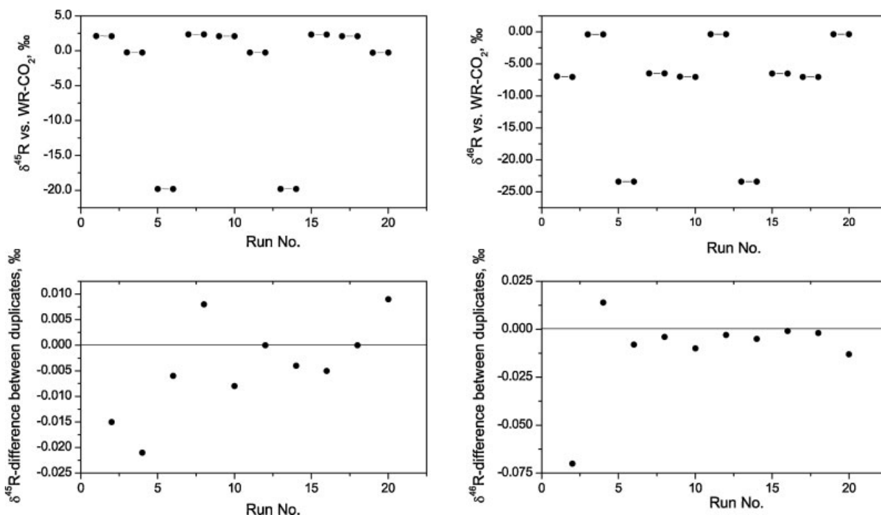
Figure 6. Test to investigate the memory effect in the CO 2 trap using runs of isotopically contrasting CO 2 -air mixtures. Extractions from each mixture were made in duplicate. The discrepancy between duplicates (lower panels) is close to zero, confirming a negligible memory in the CO 2 trap. Obvious deviation in \delta^{46}\text{R} -discrepancy on the first run (outlier) and the small positive trend in the \delta^{45}\text{R} -discrepancy are probably due to some drift in vacuum/instrumental conditions (the data are not drift-corrected). (Test performed after cleaning the system and oil-free pump installation.)
