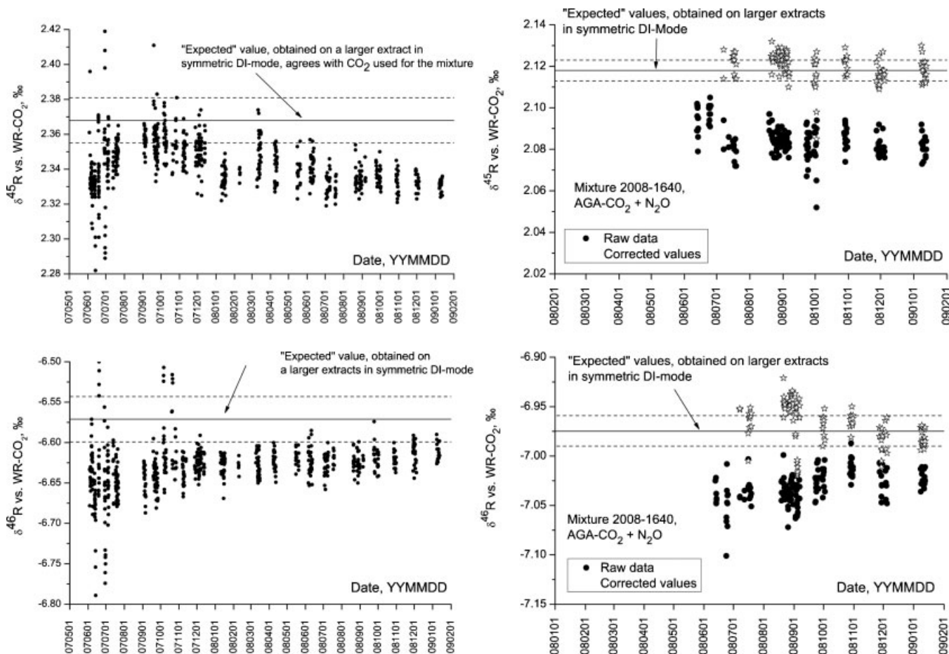
Figure 4. (a, left) Data on two (twin) AGA-CO 2 -air mixtures (without N 2 O) prepared in MPI-C, Mainz, April 2007 (10-L cylinders, Scott-Marrin Inc., filled to ~85 bar). The two cylinders have the same \delta^{13}\text{C}(\text{CO}_2) and constant offset of 0.106‰ in \delta^{18}\text{O}(\text{CO}_2) . (The data of the second/twin mixture are corrected for this offset so that data of two mixtures can be plotted together.) From the scatter, typical 1- \sigma values are estimated as about 0.01‰ for \delta^{13}\text{C}(\text{CO}_2) and 0.015‰ for \delta^{18}\text{O}(\text{CO}_2) (first guess estimation). (b, right) Mixture 2008-1640 made by Air Liquide, Belgium (50-L aluminium cylinder, ~150 bar), based on the aliquot of AGA-CO 2 in synthetic air doped with N 2 O. Shown are raw data and the corrected values (the ‘method-related’ correction based on runs on AGA-CO 2 -air mixtures). Some outliers from the expected values may be due to insufficient preconditioning of the pressure regulators and connecting lines. From the scatter, typical 1- \sigma estimated are similar to those in (a).
