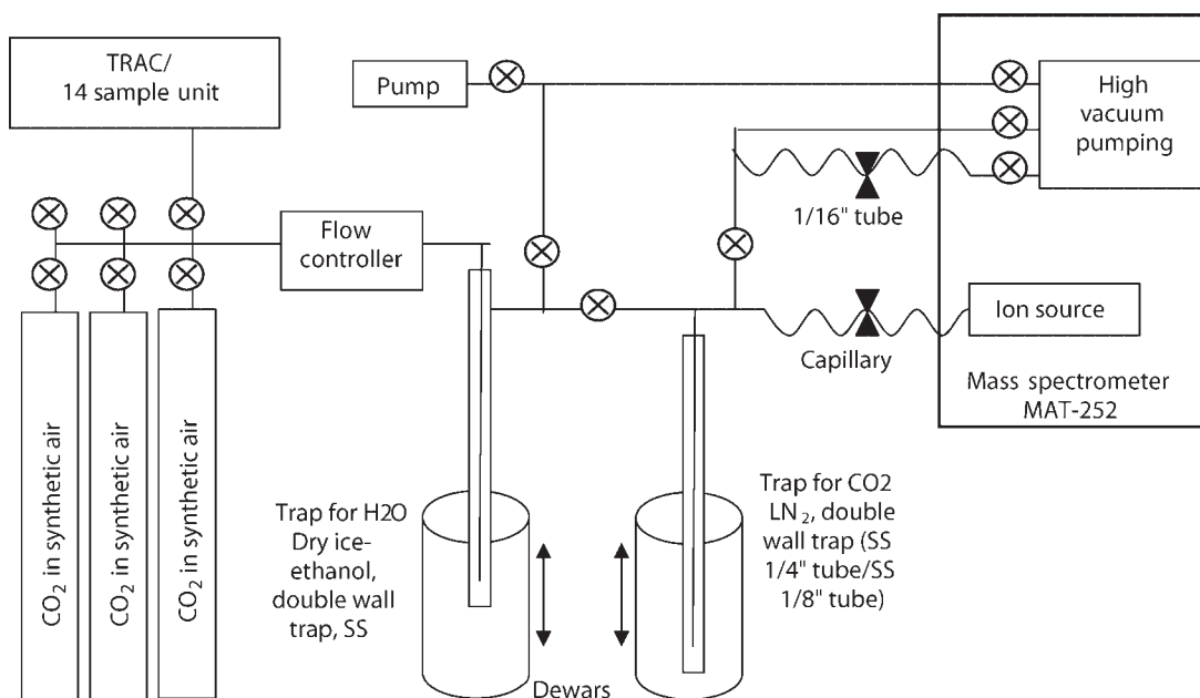
Figure 2. Schematic diagram of the CO 2 extraction line. The line is based on the system at MPI-BGC, Jena. 9
