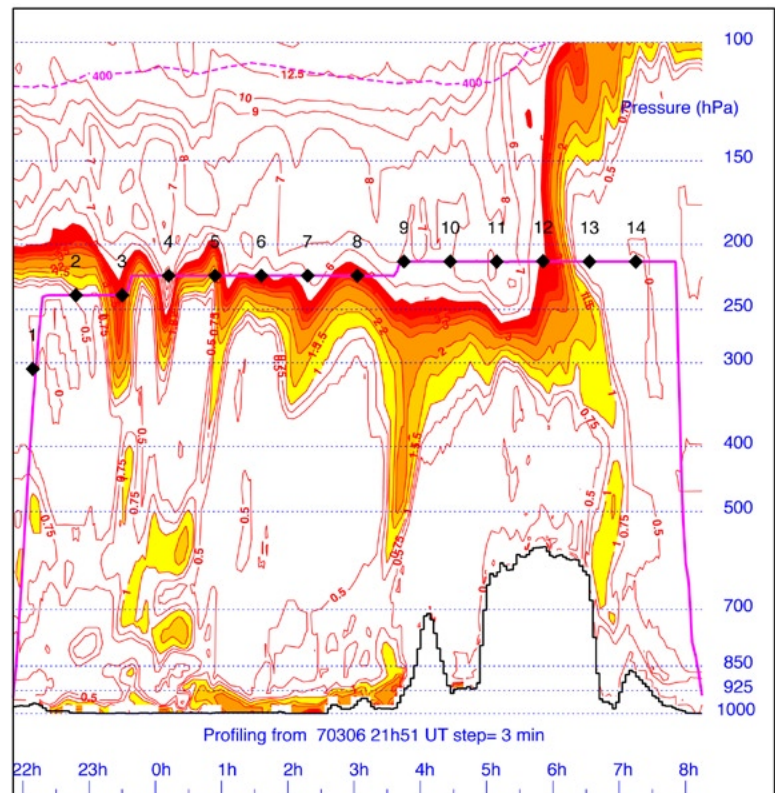
Figure 3. Vertical cross-section of the potential vorticity (PV) field along the aircraft's track for a flight from Frankfurt to Guangzhou (Cross section of 209 profiles, 7/3/2007, 0 UTC, from model level data; KNMI/ECMWF). The tropopause is highly structured, and in this particular case lowestmost stratospheric air was intercepted for about 60 % of the time. PV is, as is common, given in Potential Vorticity Units. (PV is a physical property that is largely conserved, with higher values in the stratosphere).
