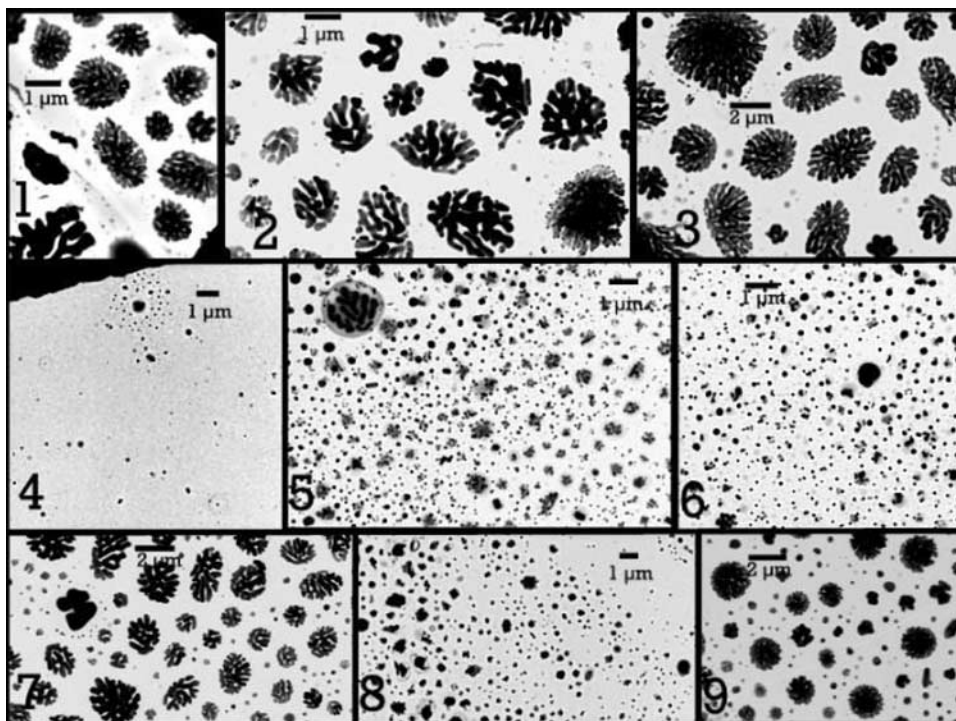
Figure 5. TEM images from the center of the impaction area of all nine samples.
