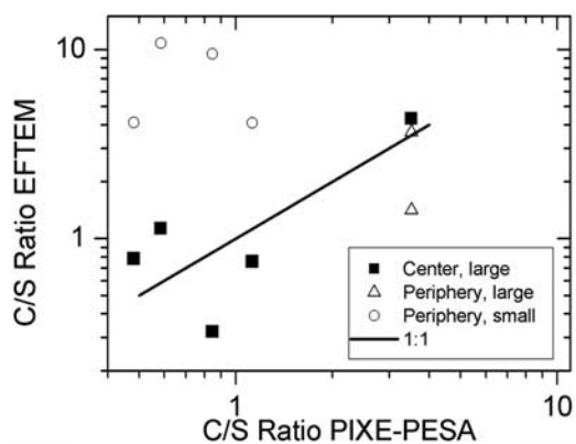
Figure 9. The carbon-to-sulfur ratio integrated from irradiated areas during EFTEM analysis according to Figure 8 related to that ratio obtained from the entire sample by PIXE and PESA. “Center, large” denotes large particles in the impaction center of the sample. “Periphery, large” and “Periphery, small” denote large and small particles at the periphery of the aerosol deposit.
