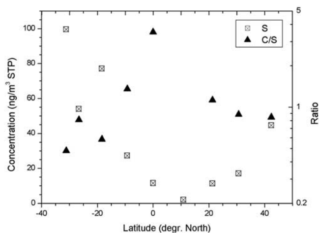
Figure 7. Concentration of sulfur ( \text{ng/m}^3 STP) and the carbon-to-sulfur mass concentration ratio (C/S) in the nine samples. The concentration of carbon in sample 4 (at latitude 10^\circ\text{N} ) was lower than the detection limit, which, expressed in terms of C/S ratio, was 2.7 for this sample.
