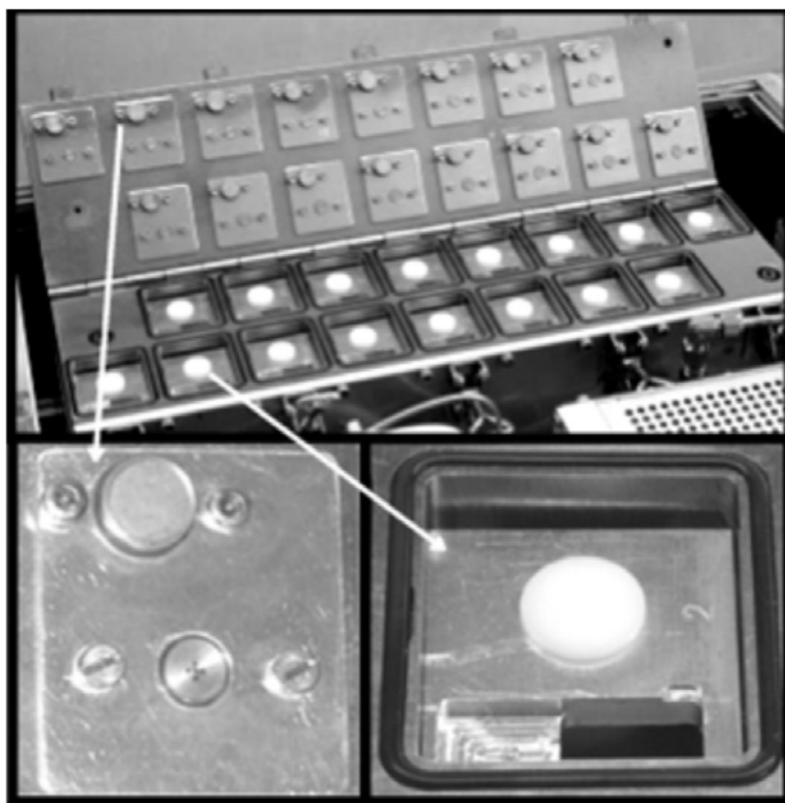
Figure 2.2: The aerosol sampler with the lid open, showing the impactors. The inserts show one channel with its nozzles (left) and the position where the film and the TEM-grids are placed (right).
